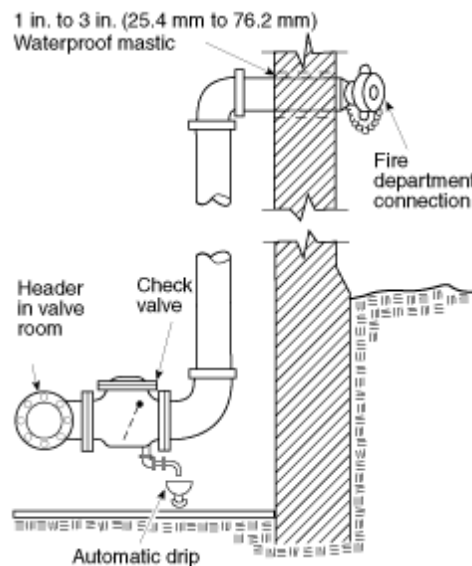
Figure A-4-3 Typical fire department connection for wet standpipes.
