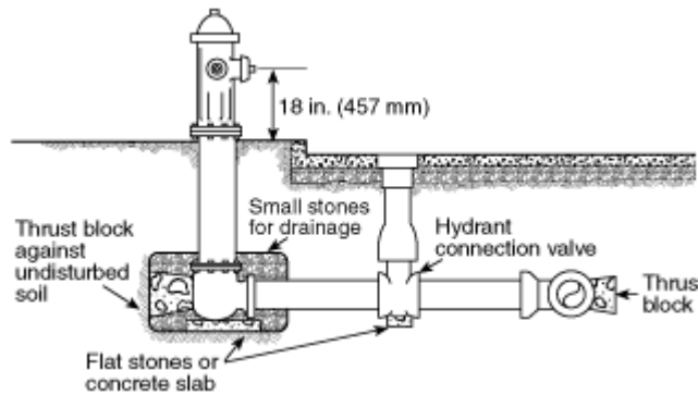
Figure A-4-5.1 Typical hydrant connection.
