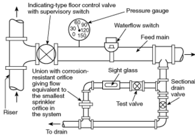
Figure A-5-9.1.3.1(b) Acceptable piping arrangement for combined sprinkler/standpipe systems.
