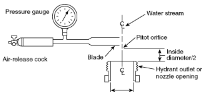
Figure B-4.2 Pitot tube position.
